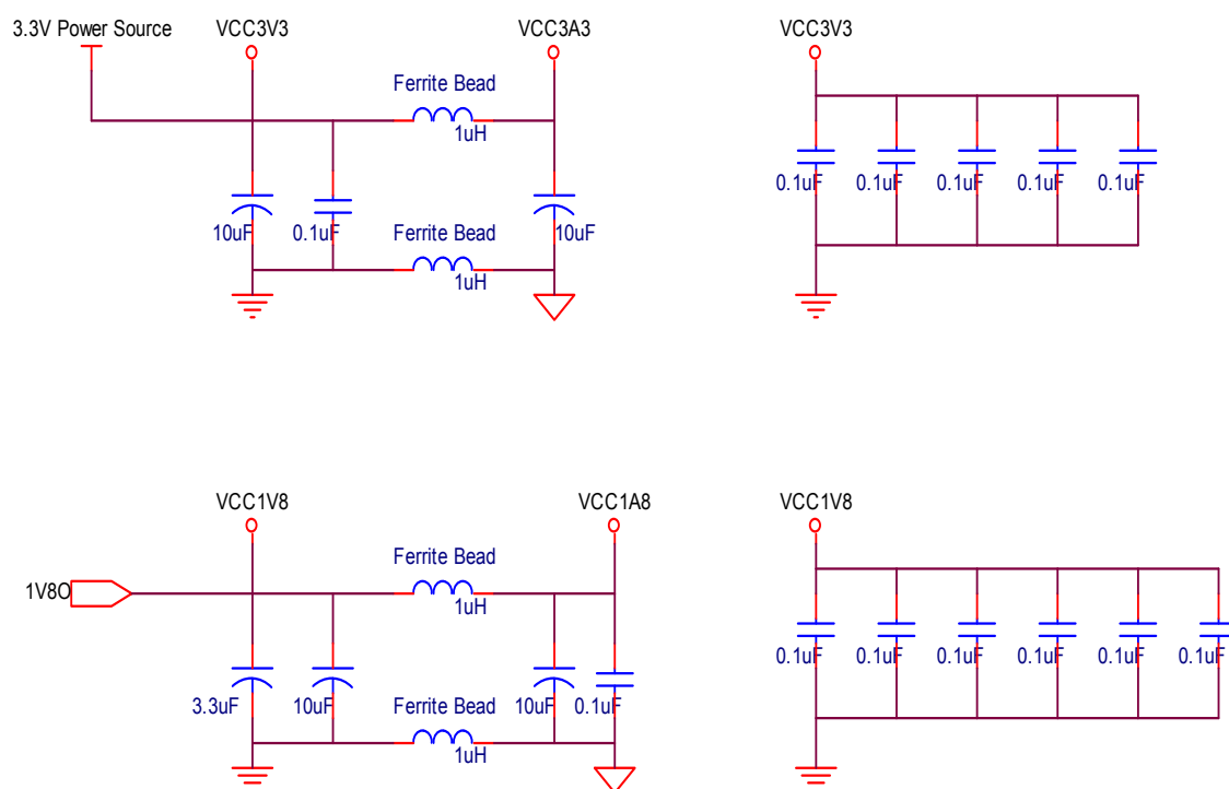
Figure 1.8 Power Design
